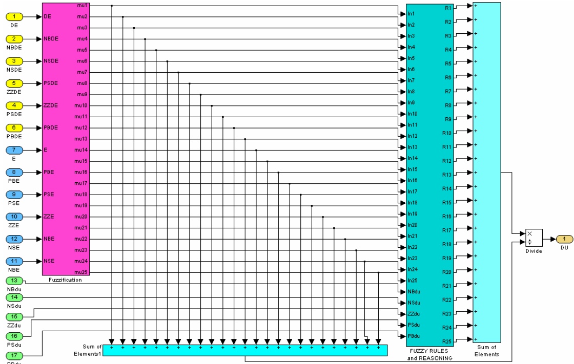
Fig. 5. The process from fuzzification to defuzzification in the FLC block.
