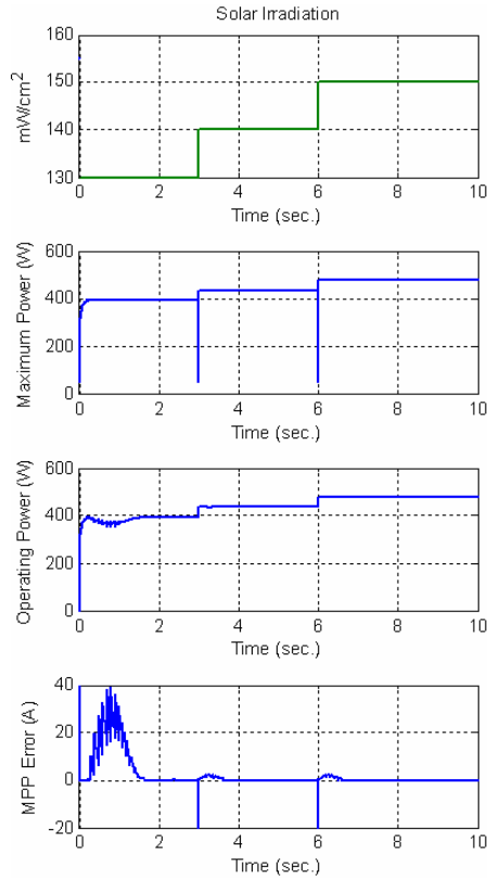
Fig. 8. Variations of the PVA power quantities as the solar irradiation level increases.
