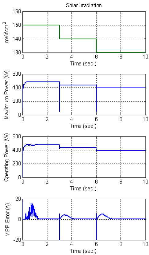
Fig. 6. Variations of the PVA power quantities as the solar irradiation level decreases.
