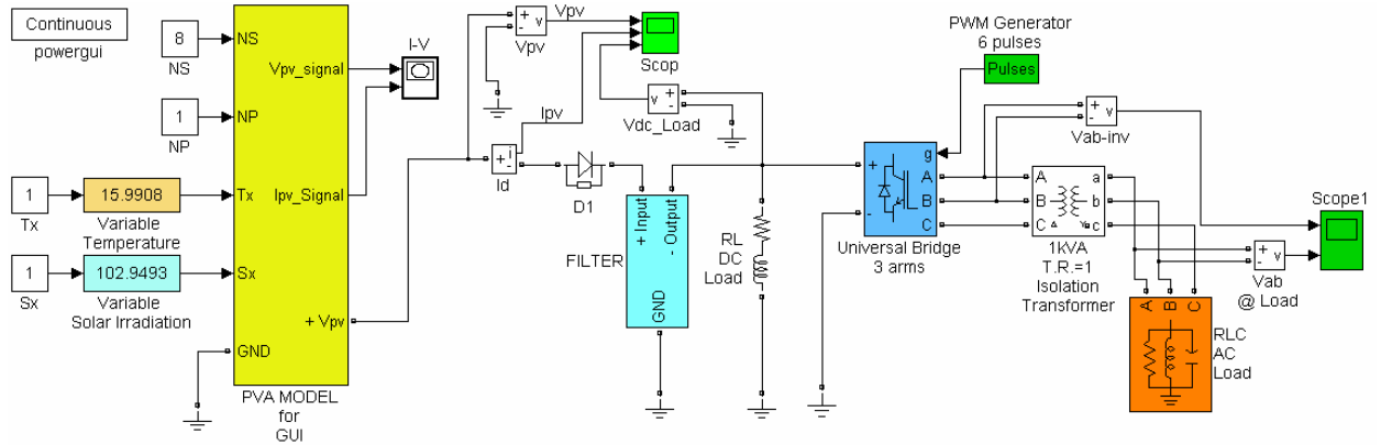
Fig. 2. Operational functional block diagram of the PVA model.
