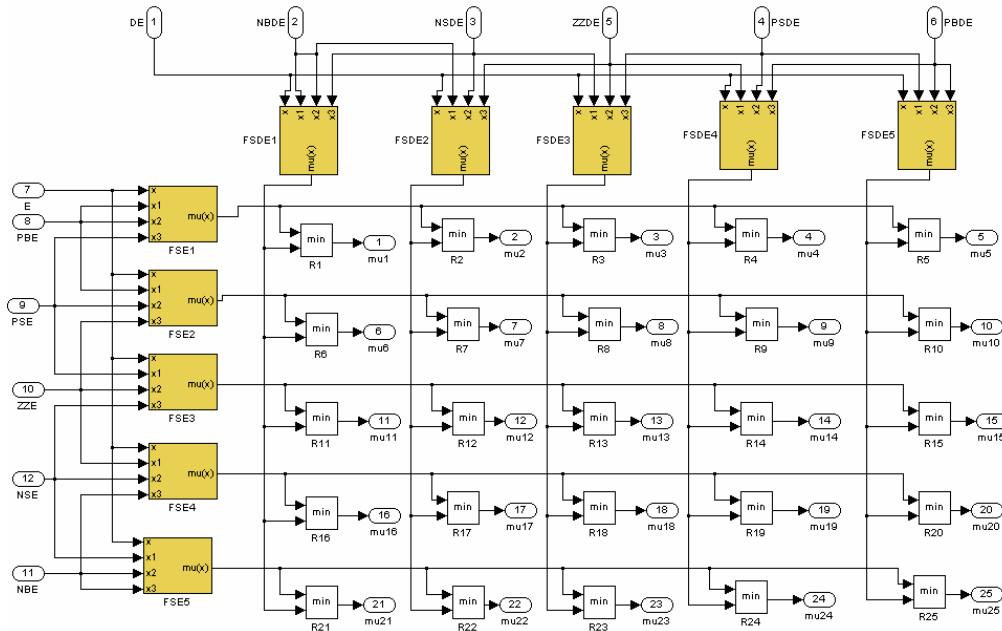
Fig. 4. The Simulink model of the Fuzzification process.
