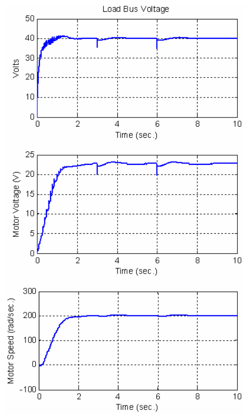
Fig. 7. Variations of the dc load bus voltage, PMDC motor voltage, and the motor speed as the solar irradiation level decreases.
