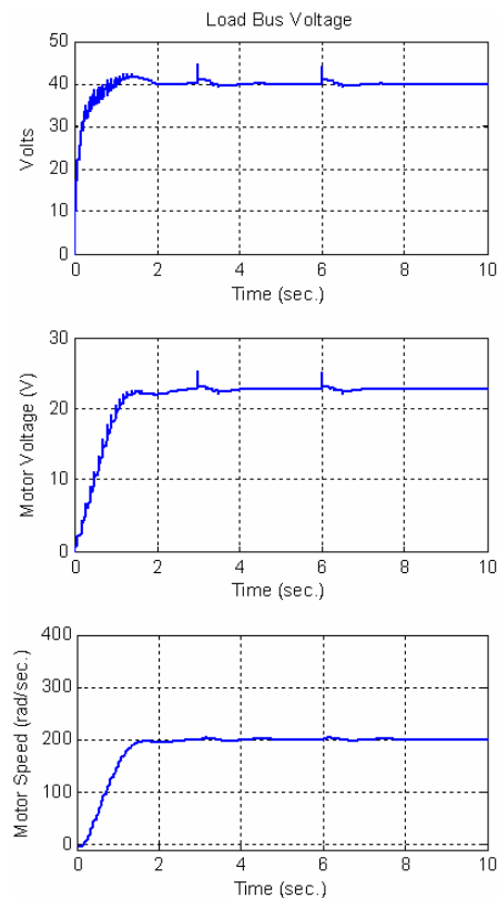
Fig. 9. Variations of the dc load bus voltage, PMDC motor voltage, and the motor speed as the solar irradiation level decreases.
