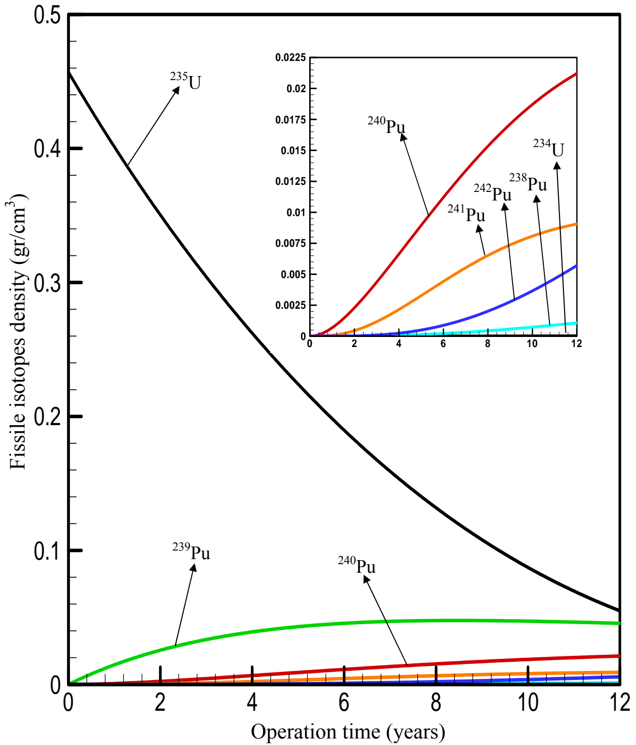
Figure 9. Density variations of the main fissionable isotopes in the FBNR fuel element
