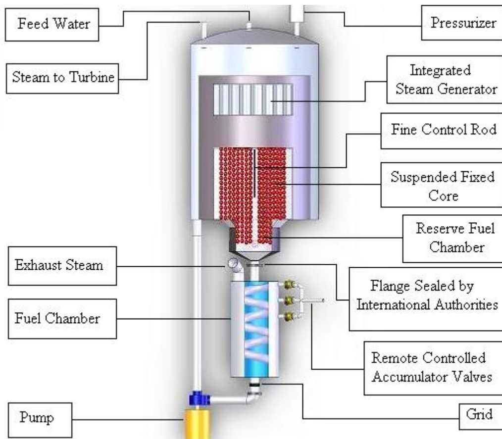
Figure 2. Schematic Design of FBNR
