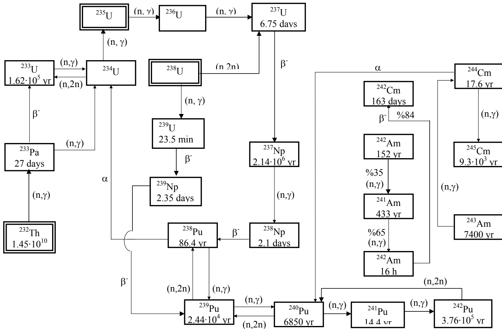
Figure 7. Major nuclear reactions and radioactive transformation processes in the course of reactor operation
