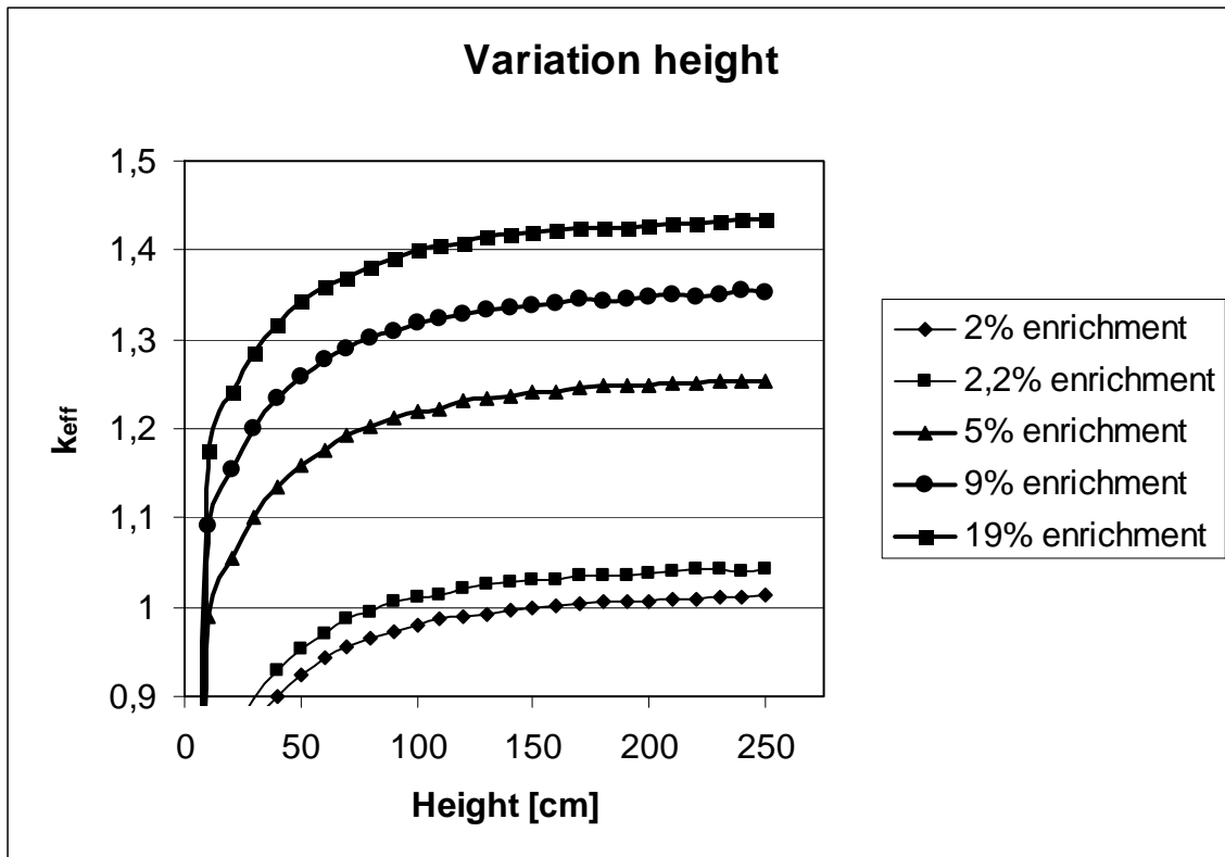
Figure 11. Variation of height for different enrichment values
