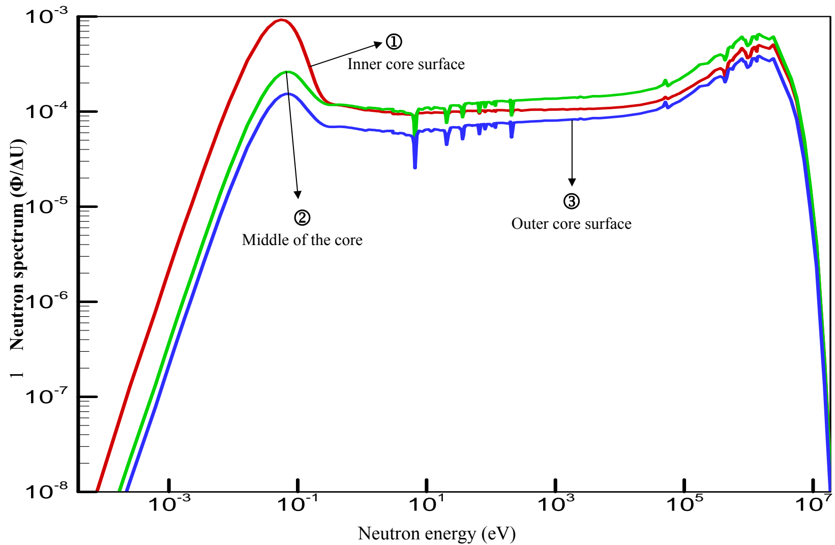
Figure 4. Neutron spectrum in the reactor
