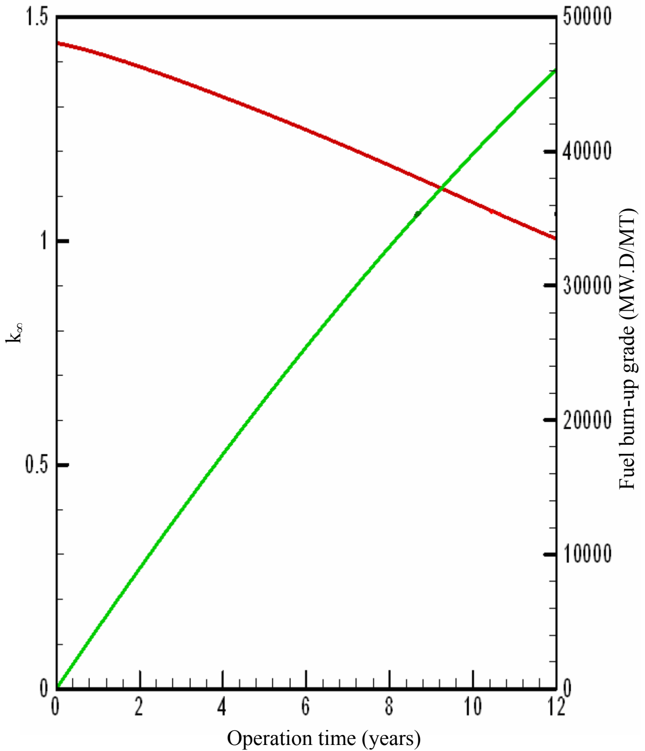
Figure 8. Temporal variation of the lattice criticality k_{\infty} and the fuel burn-up grade for FBNR fuel element
