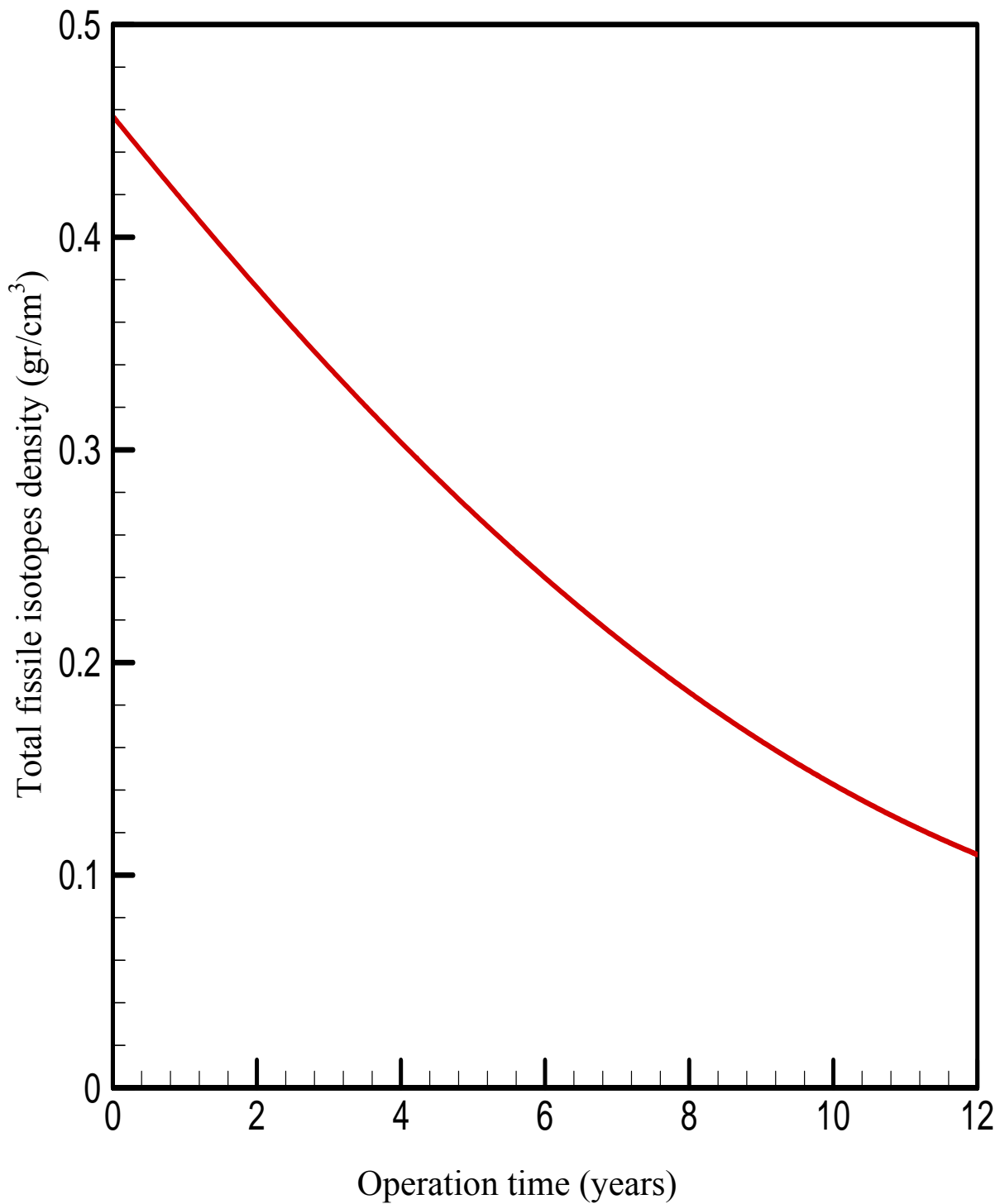
Figure 10. Temporal variation of the accumulated densities of fissile isotopes ( ^{235}\text{U} + ^{239}\text{Pu} + ^{241}\text{Pu} ) in the FBNR fuel element
