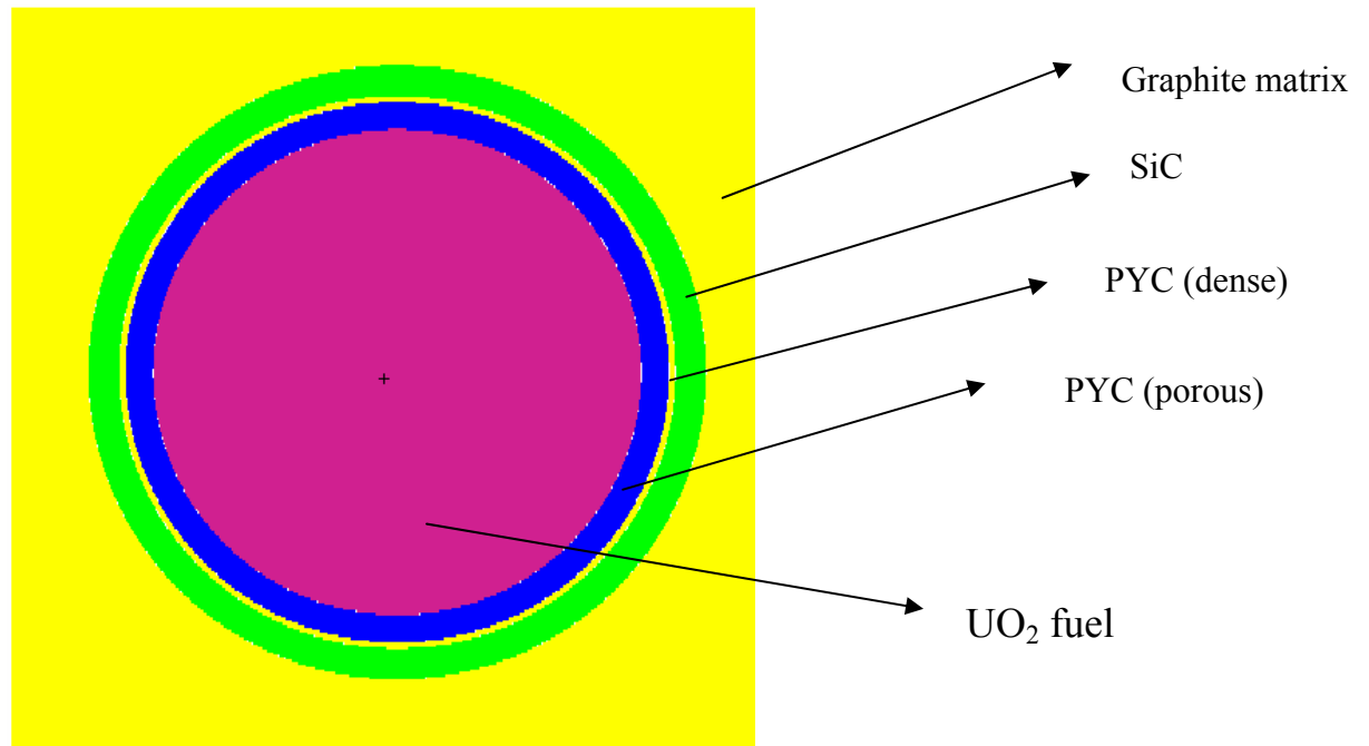
Figure 6. A typical fuel particle in the MCNP5 modeling of the FBNR unit cell
