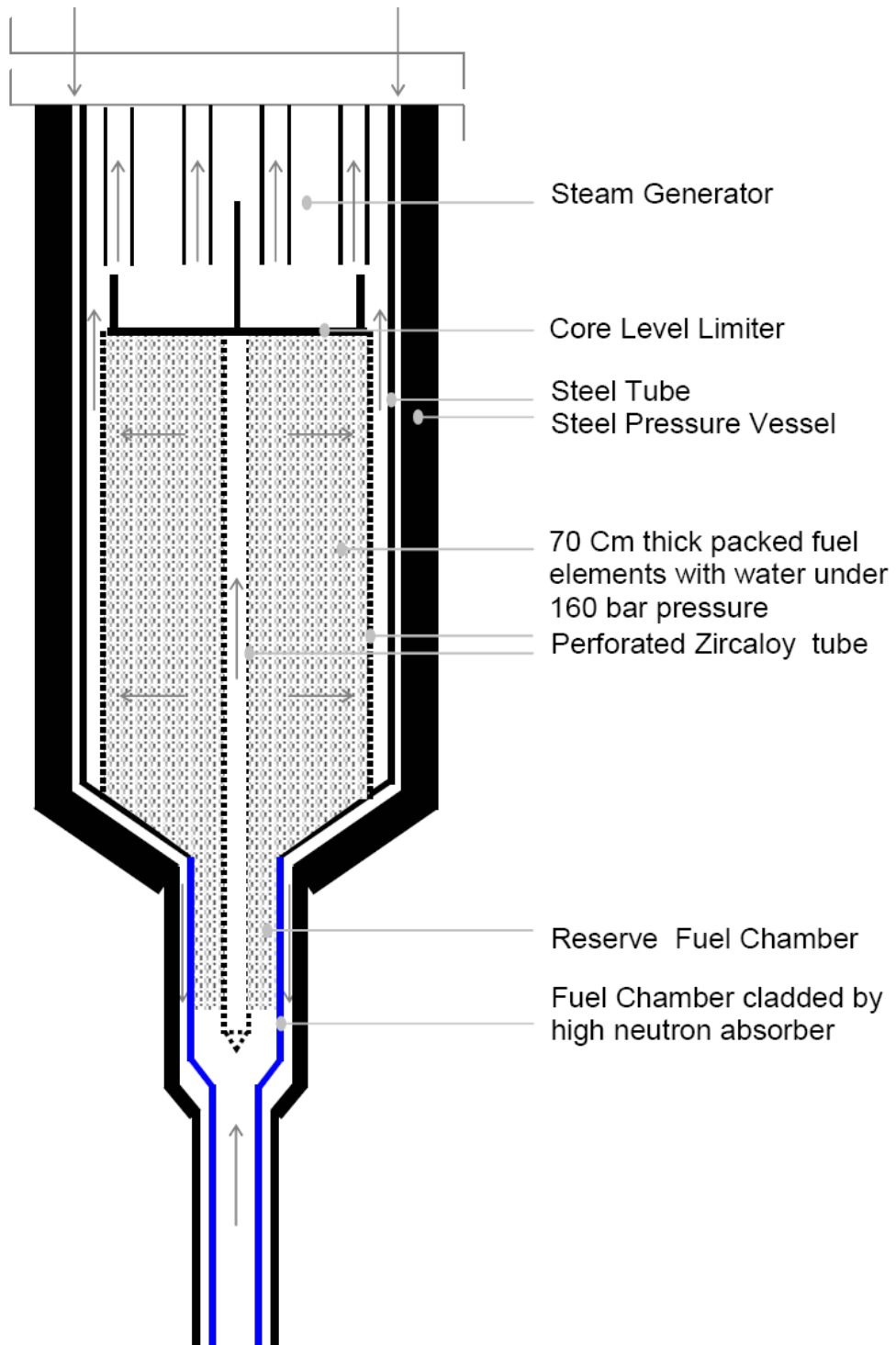
Figure 2. The basic geometrical sketch of the FBNR core
